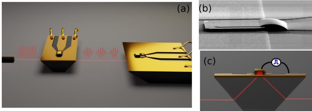
Fig. 2. (a) Sketch of our experiment comprising QC laser, Stark modulator and QC detector, all of them operating at room temperature and at the same wavelength, 9\mu\text{m} (138 meV). The laser is a commercial cw DFB QC laser (Thorlabs). The modulator and the detector have been designed, fabricated and mounted to operate at high frequency. (b) SEM image of the modulator connected via an air-bridge to the coplanar waveguide. (c) Sketch of the light coupling geometry of the Stark modulator, in order to comply with the polarization selection rule.
