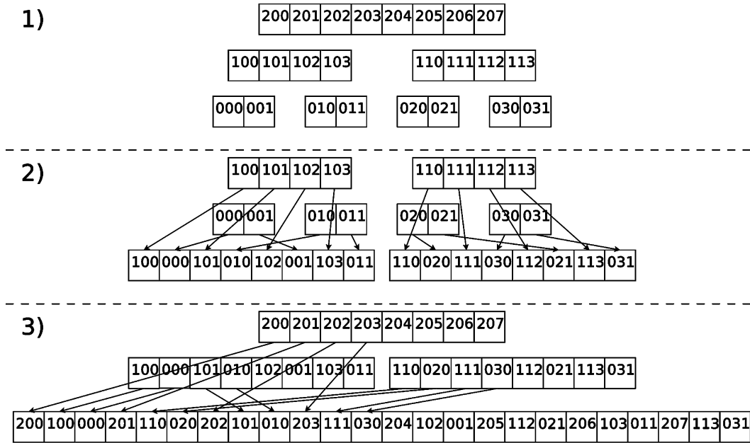
Fig.7. Interleaving process for M = 3 , L_0 = 2 . 1) The coefficients of the three blocks are given frame by frame and block by block ( XYZ is the coefficient of index m = X , p' = Y and k = Z ). 2) The frames of block 0 are interleaved two by two with the immediate upper frame of block 1. 3) The resulting two frames of interleaved coefficients are interleaved with the unique frame of block 2.
