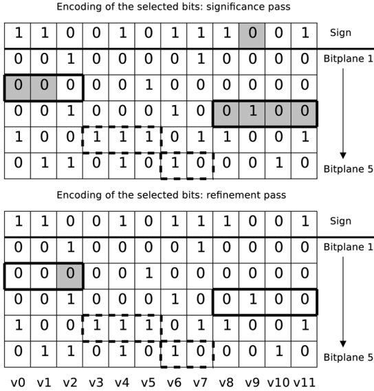
Fig.9. One iteration of the psychoacoustic bitplane encoder. Plain rectangles correspond to the level of the selected coefficients. Dotted rectangles correspond to the level of the nonselected coefficients. The two encoding passes are shown. The bits in gray correspond to the transmitted bits.
