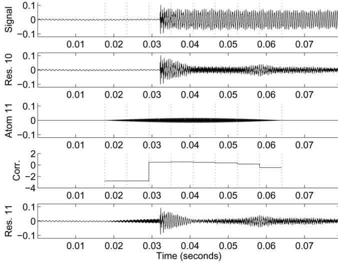
Fig.4. From top to bottom: the original signal; the residual after ten iterations; the selected atom at iteration 11; the logarithm of the absolute value of the cross-correlation between the un-windowed atom and the original signal on subframes (dotted lines); the residual after 11 iterations.
