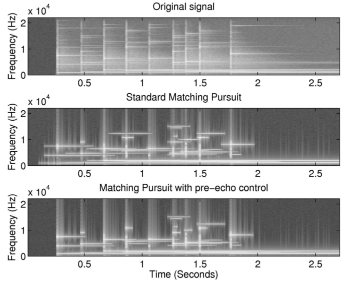
Fig.5. From top to bottom: Spectrogram of the original signal; spectrogram of the approximated signal with the standard MP and an SNR of 20 dB; spectrogram of the approximated signal with the modified MP and an SNR of 20 dB.
