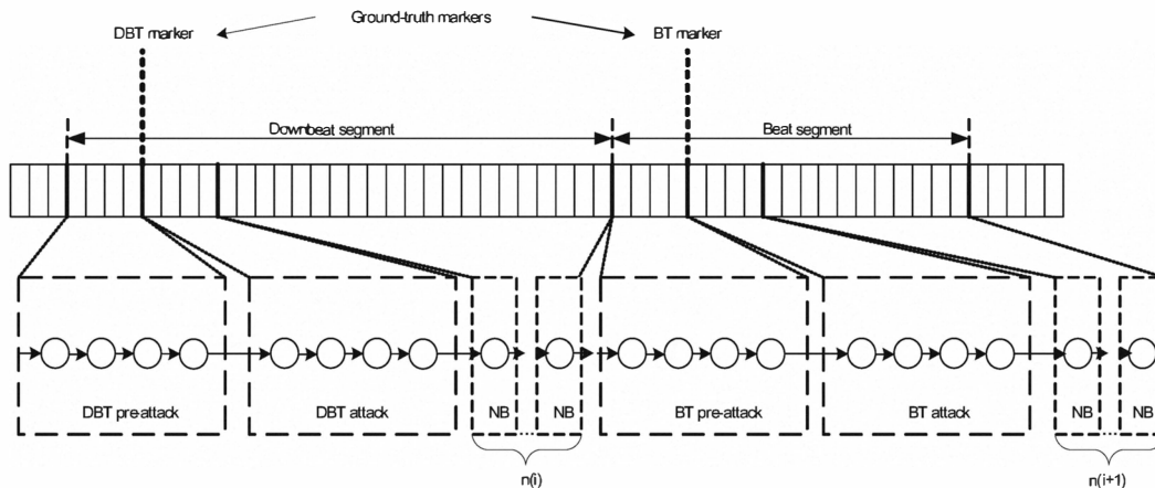
Fig. 1: Unit-based HMM training
