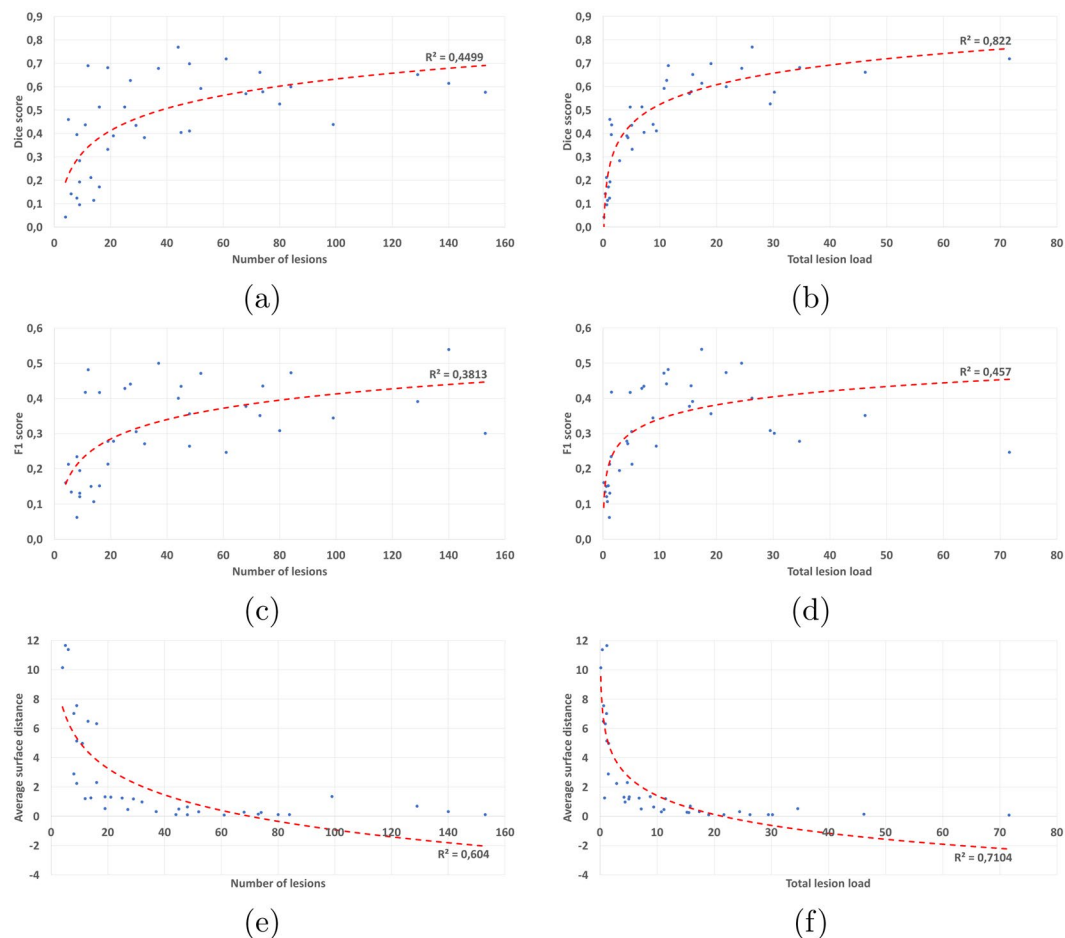
Figure 5. Link between average scores of all methods and number of lesions (first column) and total lesion load ( \text{cm}^3 , second column). First line: Dice score, second line: F_1 score, third line: average surface distance.
