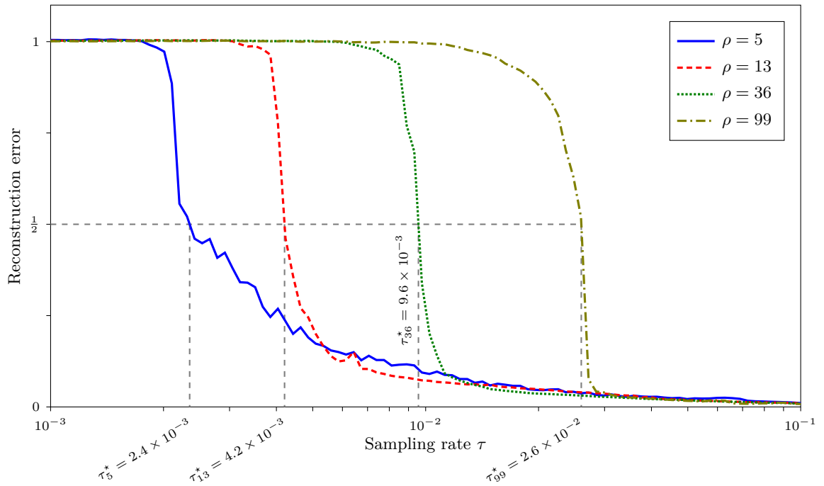
Figure 3. Evolution of the reconstruction error for four one-disk images with various radius \rho , and the associated critical sampling rates \tau^* computed from the curves.
