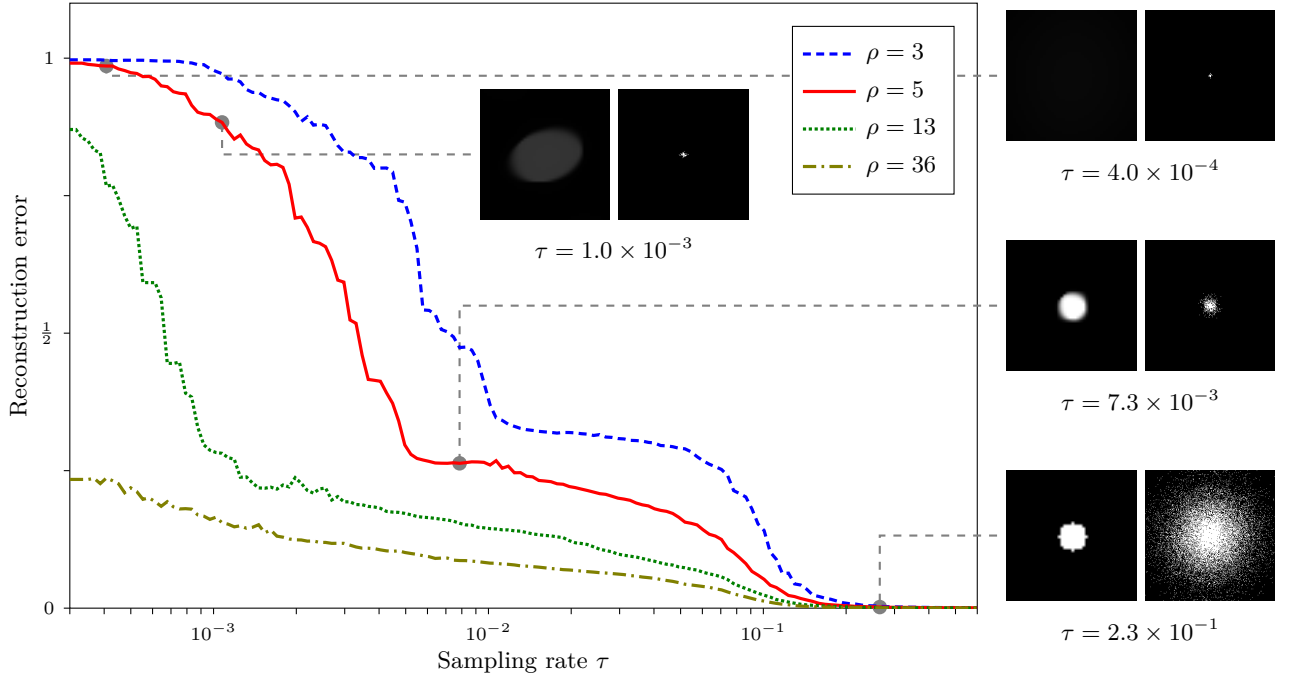
Figure 7. Evolution of the reconstruction error for four one-disk images with various radius \rho , when sampled according to a Gaussian sampling strategy. We presents also four zoomed reconstructions of the \rho = 5 one-disk test image, with their associated sampling patterns. The reconstructed image obtained for \tau = 2.3 \times 10^{-1} is almost identical to the original image.
